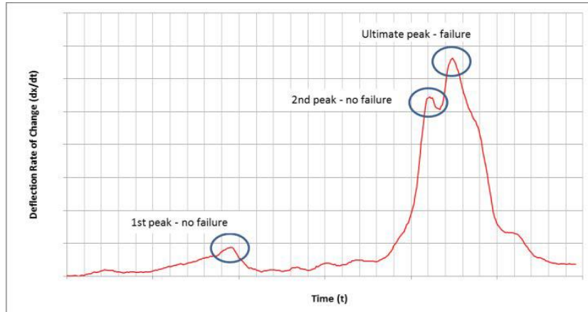
FIGURE A2--DEFLECTION RATE CURVE
